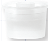
11188 Press in Bottle Adapter 0.68 inch OD (17 mm) LDPE
