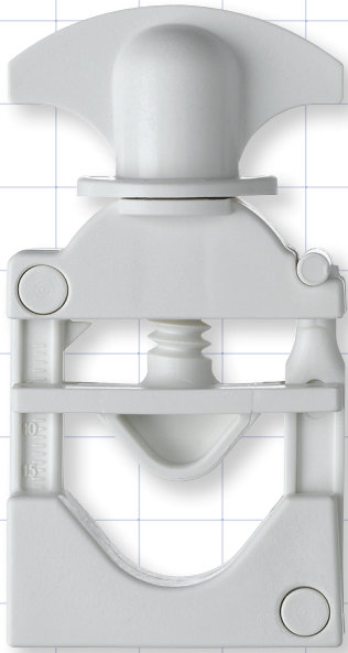
51613 Biovalve™ Fits 1/8 inch - 3/8 inch OD Tubing (0.125 inch - 0.375 inch; 3.2 mm - 9.5 mm) Glass Reinforced Nylon
