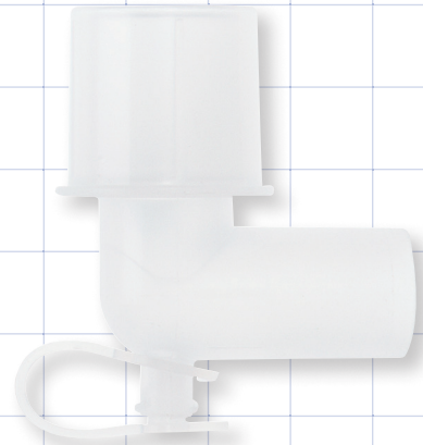
55119 15 mm ID/22 mm OD x 15 mm OD; 4.1 mm ID Pressure Port with Cap LDPE, PP
