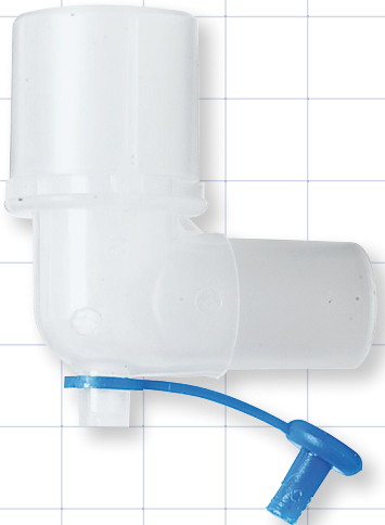
51033 15 mm ID/22 mm OD x 15 mm OD; Female Luer Lock with Cap LDPE, PP
